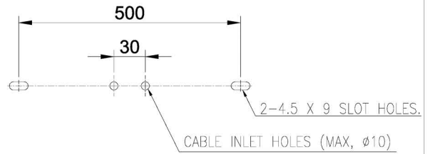
SETTING DIMENSION
